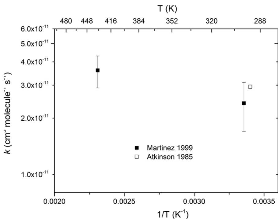
Rate coefficients for \text{NO}_3 + \gamma -terpinene
